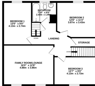
1ST FLOOR 770 sq.ft. (71.5 sq.m.) approx.
