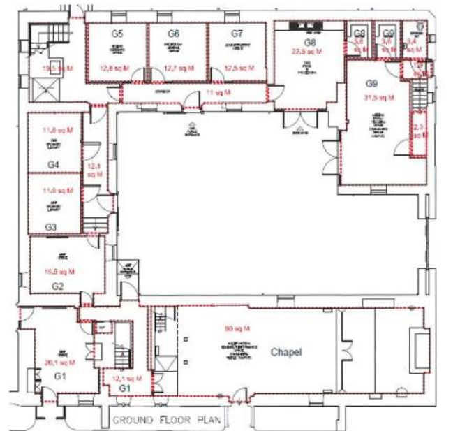
Stable Block - Indicative plans
