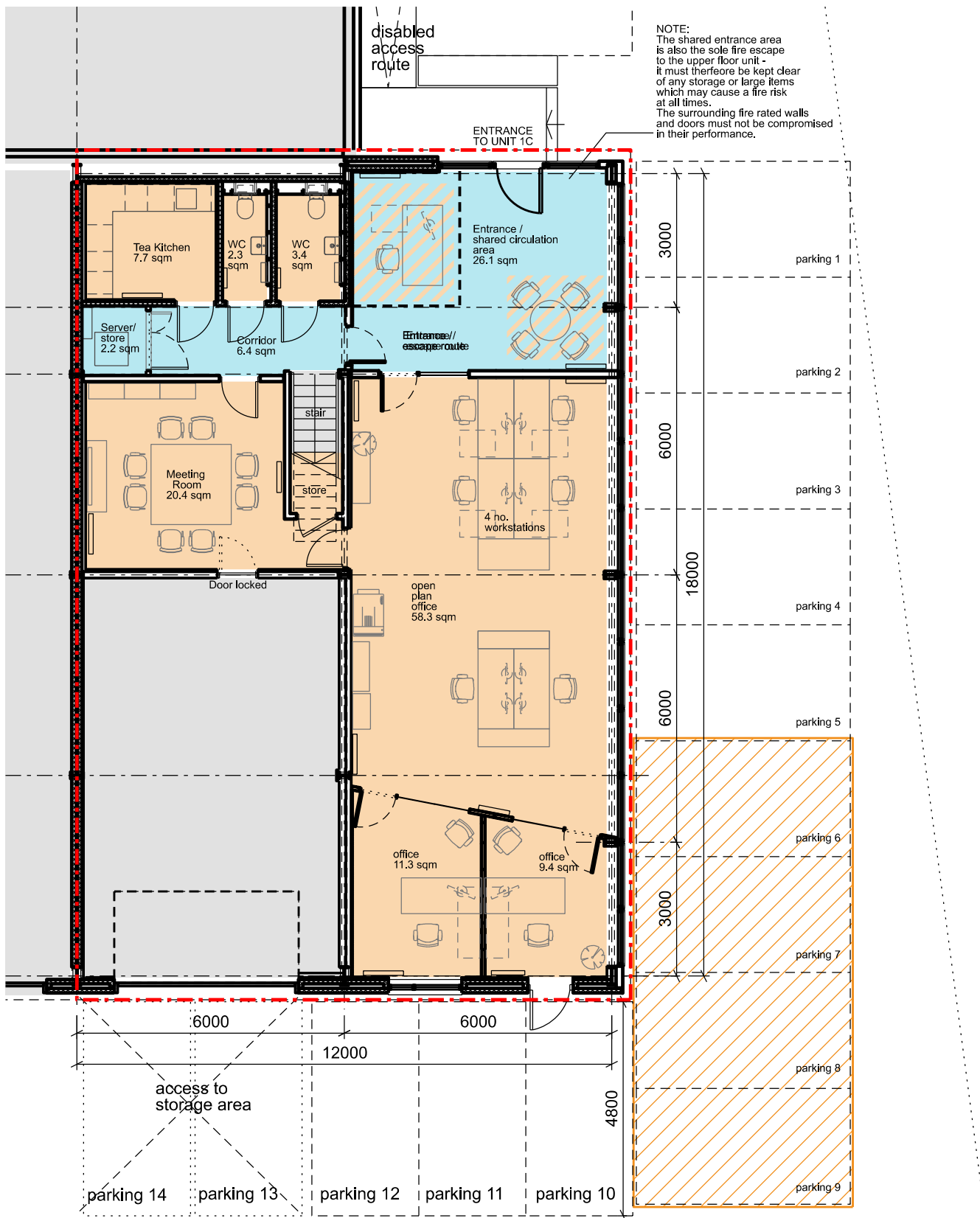
LEGEND FOR GROUND FLOOR LICENCE PLAN
