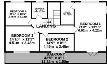
1ST FLOOR 942 sq.ft. (87.5 sq.m.) approx.
